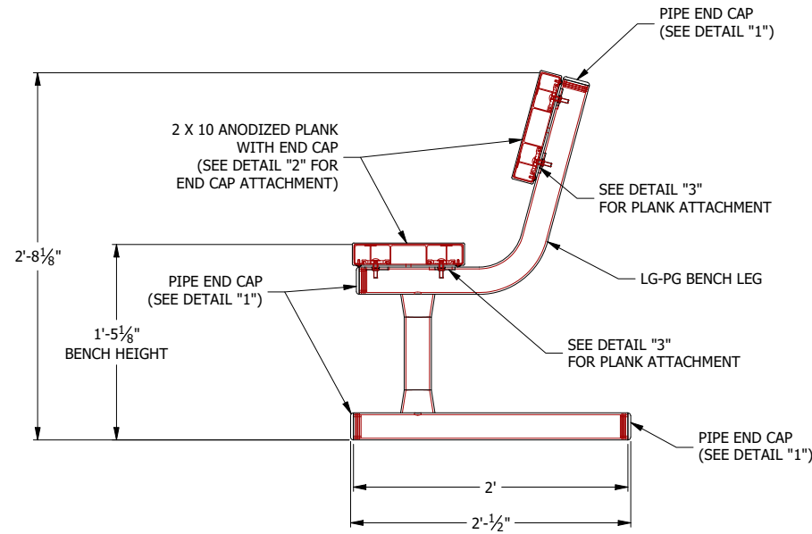
END VIEW
